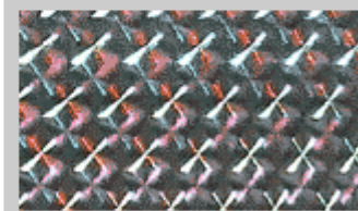
Diffraction Tricle
